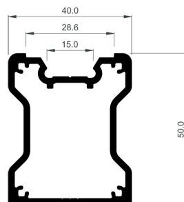
Reinforcement 40x50mm
