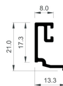
Glazing bead 8mm Double glazed
