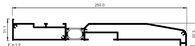
Cill 250mm
