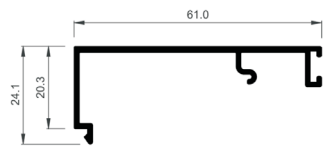
Frame cover for fixed light
