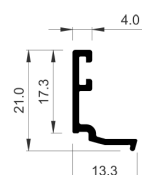
Glazing bead 4mm Triple glazed
