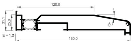
Cill 180mm
